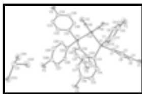
Fig. 1. The molecular structure of the title compound. Hydrogen atoms were omitted for clarity. The displacement ellipsoids were drawn at the 50% probability level.
